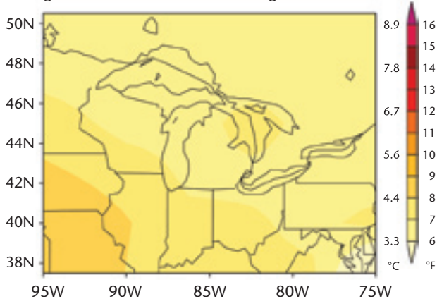
2070–2099 Summer (JJA) Temperature for Low Emissions Change Relative to 1961–1990 Average
