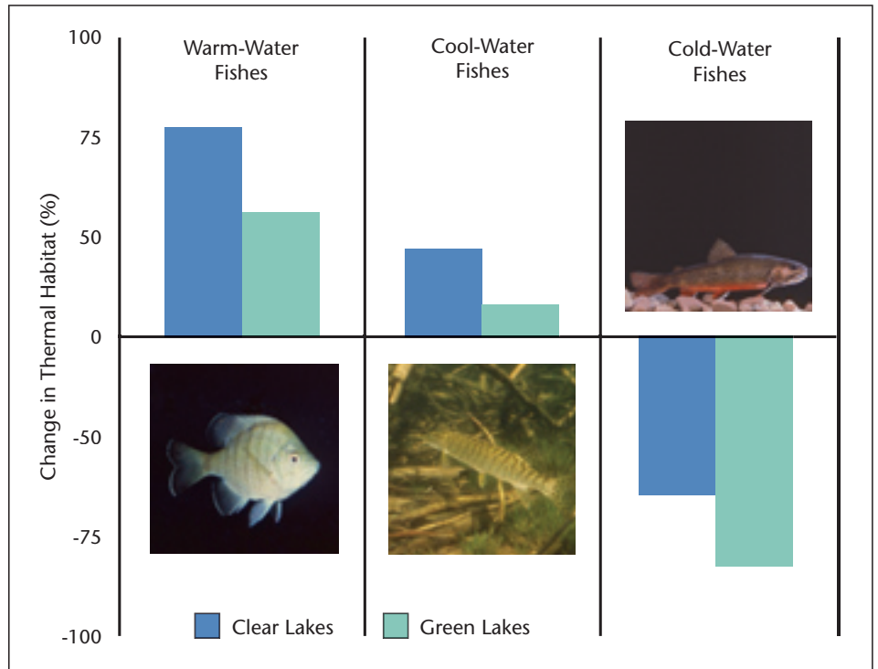
FIGURE 24 Water Temperature and Fish Distribution Changes
