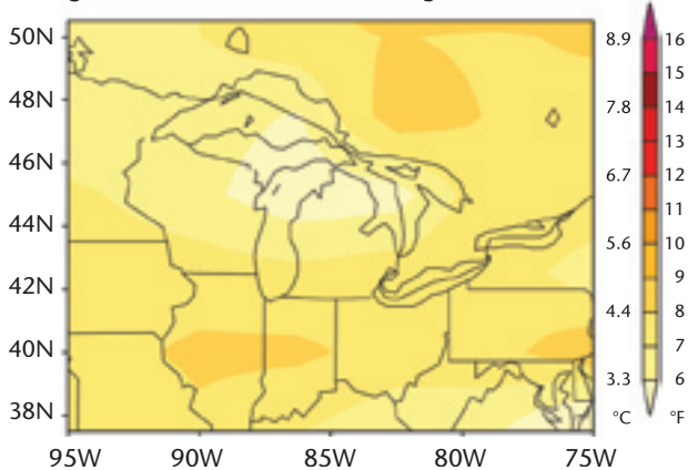
2070–2099 Winter (DJF) Temperature for Low Emissions Change Relative to 1961–1990 Average
