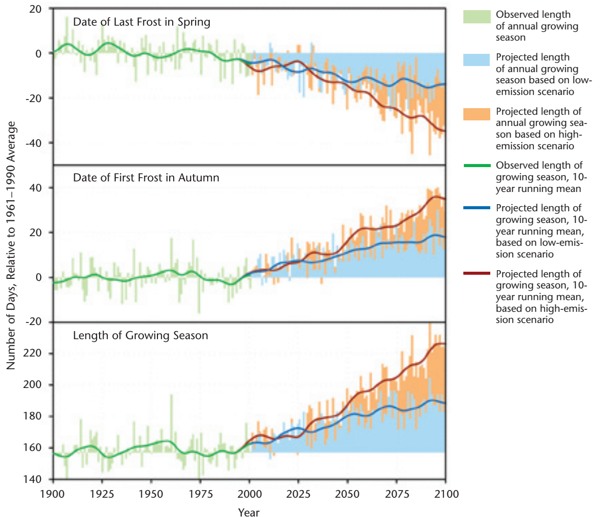
FIGURE 11 Growing Season in the Great Lakes Region (Observed and Projected Changes, 1900–2100)
