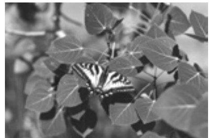
FIGURE 28 Range Shifts of the Canadian Tiger Swallowtail
