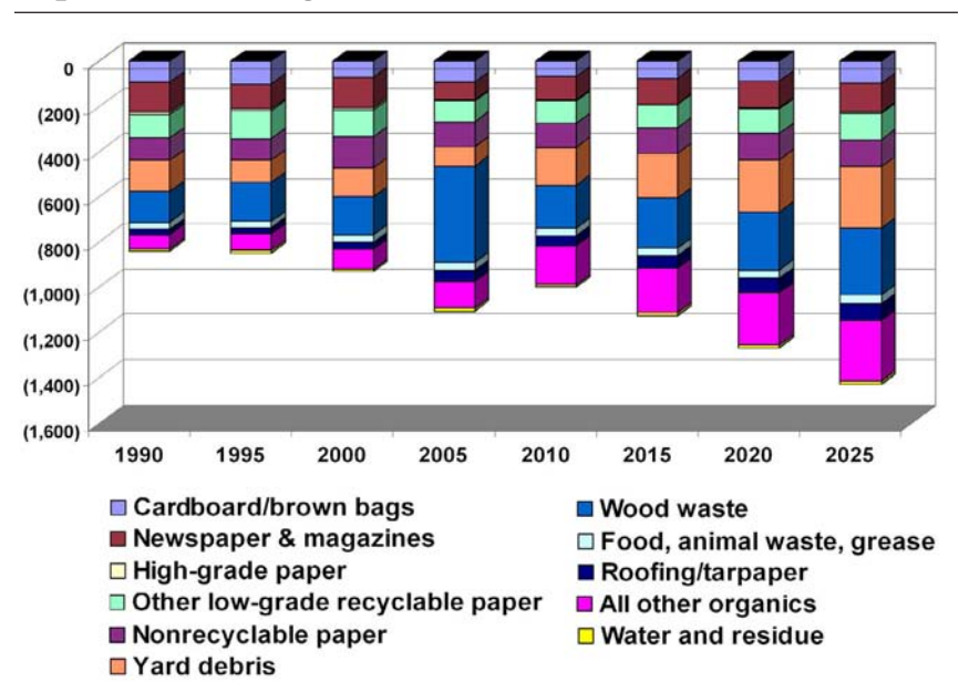
Figure 22: Thousand Metric Tons of Carbon (in CO 2 e) Sequestered in Oregon Landfills
