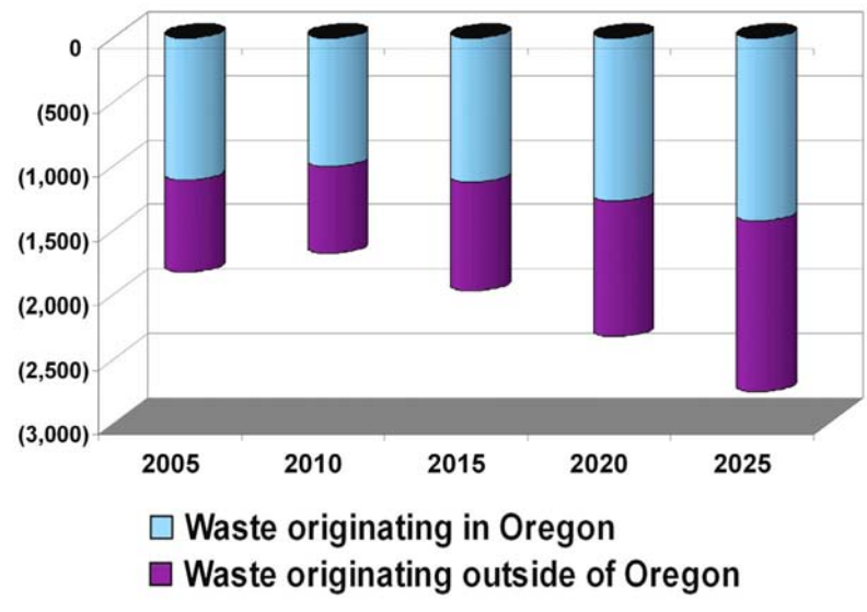
Figure 23: Imported Waste Impacts on Sequestered Carbon in Oregon Landfills (Thousand Metric Tons COe)
