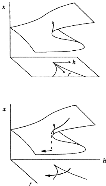
Fig. 1. Diagram of a cusp catastrophe fold. The 3-D projection (top panel) shows the equilibrium space for a nonlinear system; when projected onto a 2-D map, it shows a bifurcation. In certain parts of state space, rapid movement from one equilibrium state to another can occur. (Source: Strogatz 1994).
