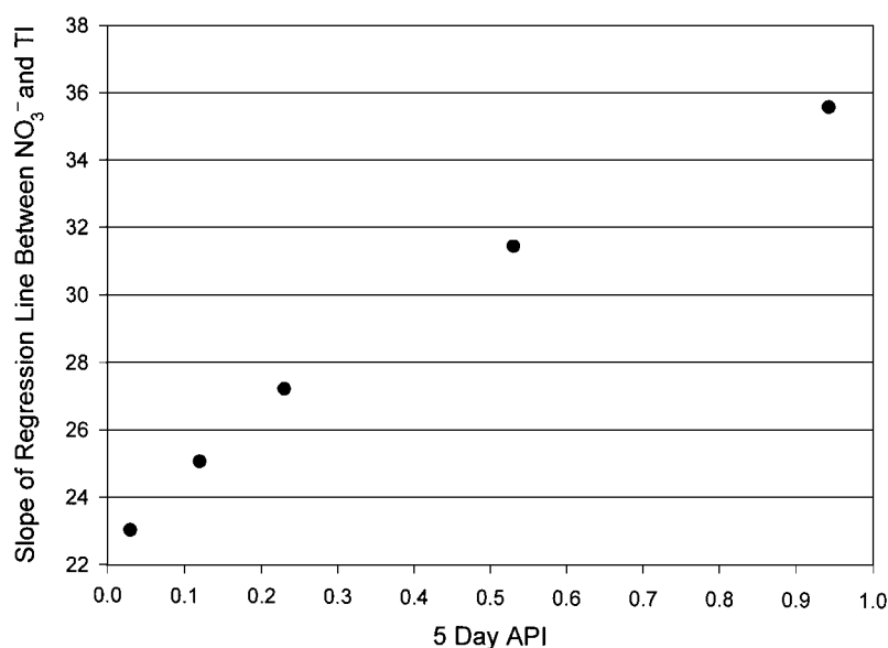
Figure 7. The NO 3 - concentration–TI slope as a function of the 5 day API for the five storms analysed
