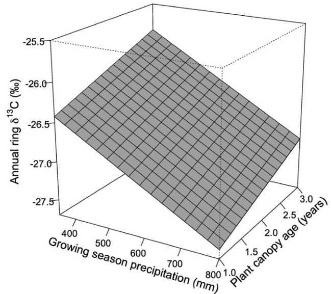
Fig. 4 – Response surface plot of the best linear mixed-effects model predicting tree-ring \delta^{13}\text{C} value based on growing season precipitation, and plant canopy age. The formula for this model is: \delta^{13}\text{C} = -25.80 - 0.0026 * \text{precipitation} + 0.28 * \text{stem age} . Wood becomes more isotopically enriched with plant age and in years with lower precipitation.
