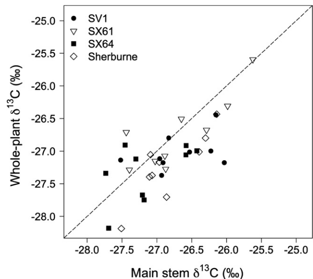
Fig. 2 – Relationship between largest stem and whole-plant \delta^{13}\text{C} values. The dotted 1:1 line indicates a null hypothesis of no difference; points that fall below the line represent stems that are more enriched in ^{13}\text{C} than the whole-plant.
