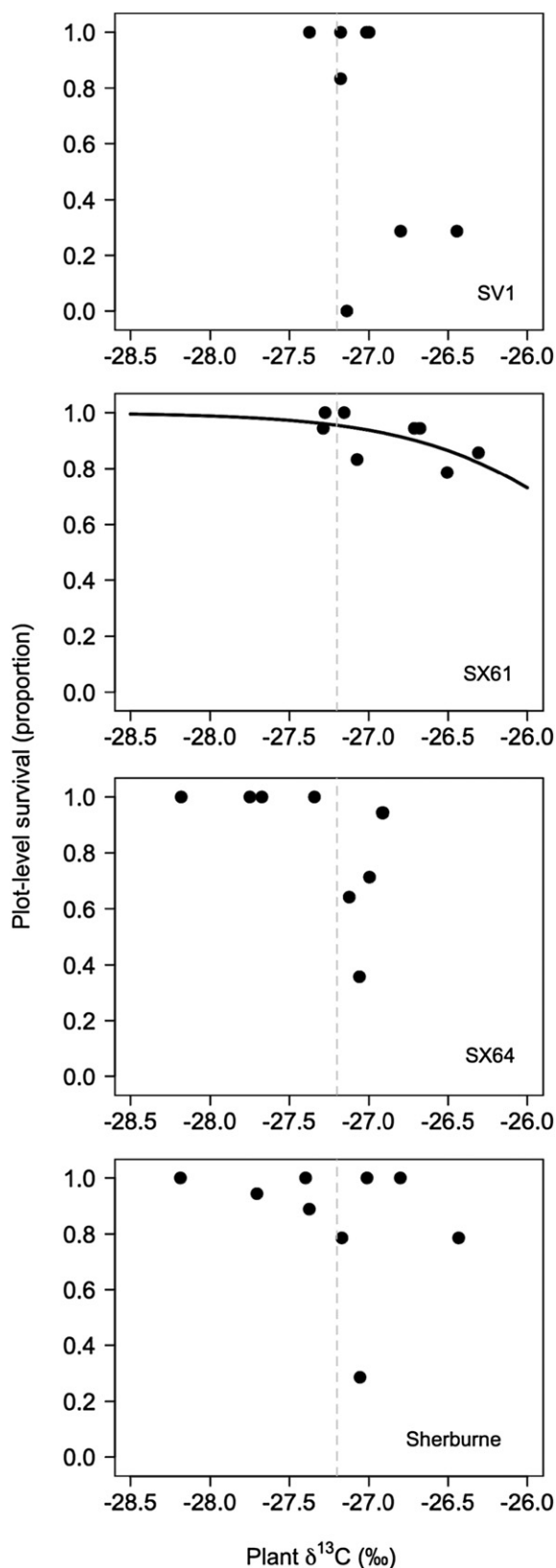
Fig. 6 – Relationship between plot-level survival and \delta^{13}\text{C} values of representative surviving plants from those plots. Plots with more isotopically enriched plants ( > -27.2 ‰, indicated by points to the right of the dotted lines) had more variable survival across all varieties; however, only variety SX61 showed a significant predictive relationship
