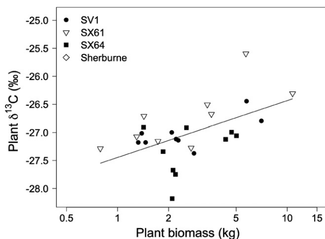
Fig. 5 – Relationship between whole-plant \delta^{13}\text{C} values and aboveground biomass (log scale). The solid line represents the best fit from a mixed-effects model with variety nested within site as random factors and biomass as the sole fixed effect ( t = 3.24, p < 0.01 ). The correlation between observed and predicted values from the model is r = 0.81 .
