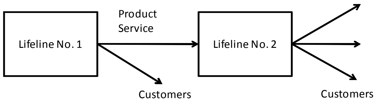
Figure 4-1 First Order-Dependency
