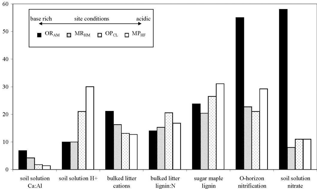
FIG. 2. Summary of site conditions, litter quality, and nutrient cycling processes at four Adirondack northern hardwood forest sites. Study sites have been ordered in relation to site conditions. Response variables are: Ca:Al in shallow (15 cm) soil solution; H + concentration in shallow soil solution ( \mu\text{eq L}^{-1} ); bulked leaf litter total cation content ( \text{mg g}^{-1} dry wt); bulked leaf litter lignin:N; sugar maple litter lignin content (percent); O-horizon net nitrification rates ( \mu\text{mol N g}^{-1} dry wt soil \text{yr}^{-1} ); \text{NO}_3^- concentration ( \mu\text{eq L}^{-1} ) in soil solution below rooting zone (50 cm).
