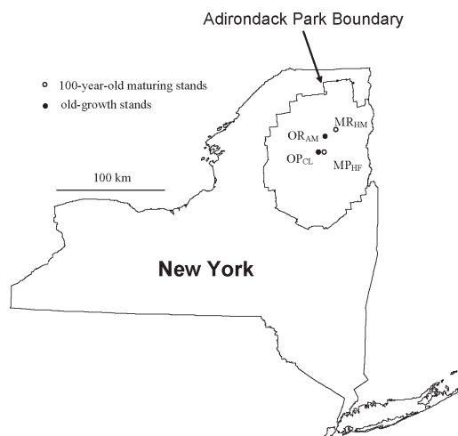
FIG. 1. Location of the four northern hardwood forest study sites in Adirondack Park, New York: Ampersand Mountain ( \text{OR}_{\text{AM}} ), Hennessy Mountain ( \text{MR}_{\text{HM}} ), Catlin Lake ( \text{OP}_{\text{CL}} ), and Huntington Forest ( \text{MP}_{\text{HF}} ). Subscripts are explained in Methods: Research Setting and Study Sites.
