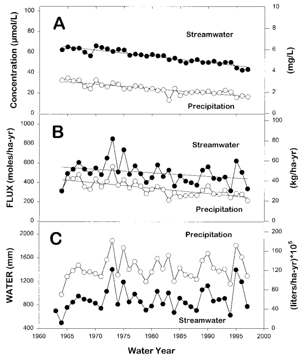
Figure 3. A. Annual, volume-weighted concentrations of \text{SO}_4^{2-} in bulk deposition ( \text{--}\circ\text{--} ) and streamwater ( \text{--}\bullet\text{--} ) for W6 of the HBEF during 1964–1997. The probability for a larger F-ratio for both regression lines is p < 0.001 ; the r^2 for bulk precipitation is 0.72, and for streamwater is 0.87. B. Annual inputs of \text{SO}_4^{2-} in bulk deposition ( \text{--}\circ\text{--} ) and outputs in stream water ( \text{--}\bullet\text{--} ) for W6 during 1964–1997. The probability of a larger F-ratio for the regression line for stream water is p = 0.067 , r^2 = 0.10 ; and for bulk deposition is p < 0.001 , r^2 = 0.48 . C. Annual amount of precipitation ( \text{--}\circ\text{--} ) and streamflow ( \text{--}\bullet\text{--} ) for W6 of HBEF during 1964–1998.
