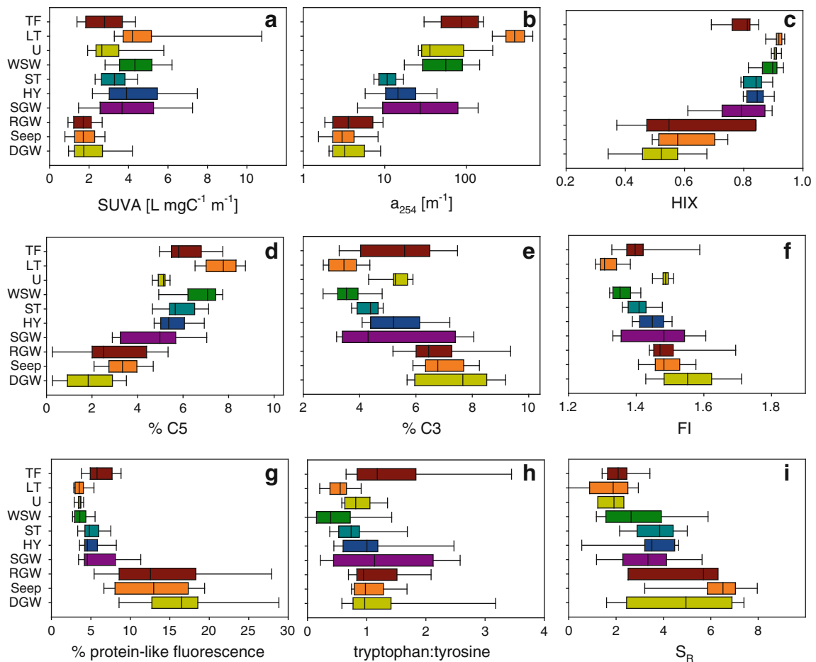
Fig. 3 Values for DOM quality indices for various watershed sources (line = median, box upper and lower bound = 25% and 75%, whiskers = 10% and 90%). These indices include: Specific UV absorbance (SUVA), absorption coefficient a_{254} , humification index (HIX), Cory and McKnight (2005) model
