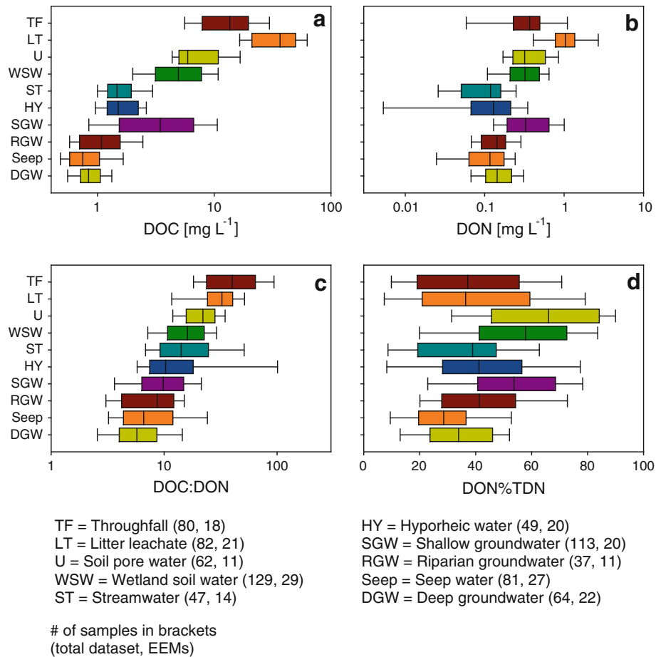
Fig. 2 Concentrations of: a DOC ( \text{mg L}^{-1} ); b DON ( \text{mg L}^{-1} ); c DOC:DON ratios and d DON as a % of total dissolved N (TDN) for the various watershed sources ( line median, box upper and lower bound = 25% and 75%, whiskers = 10% and 90%). Sample numbers are indicated
