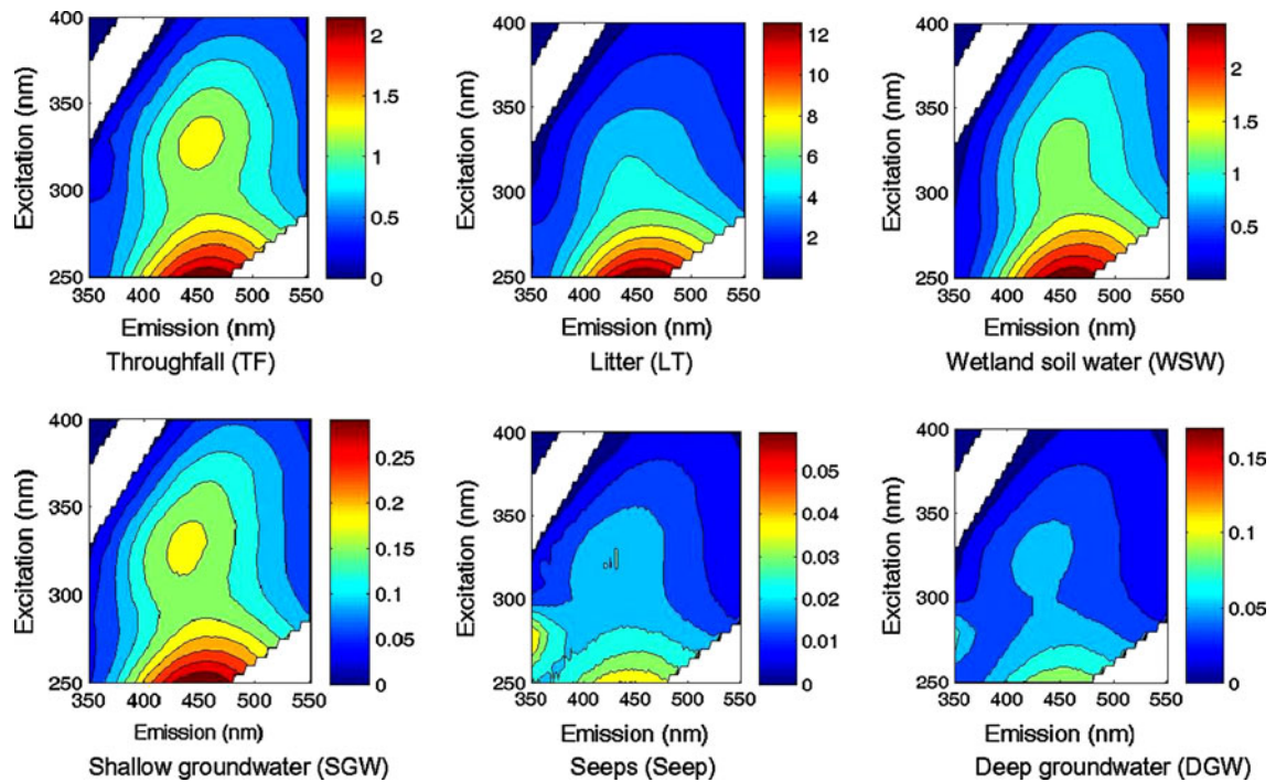
Fig. 4 Excitation-emission matrices (EEMs) for selected watershed sources highlighting the shift in fluorescence. Throughfall and litter samples correspond to event of October
