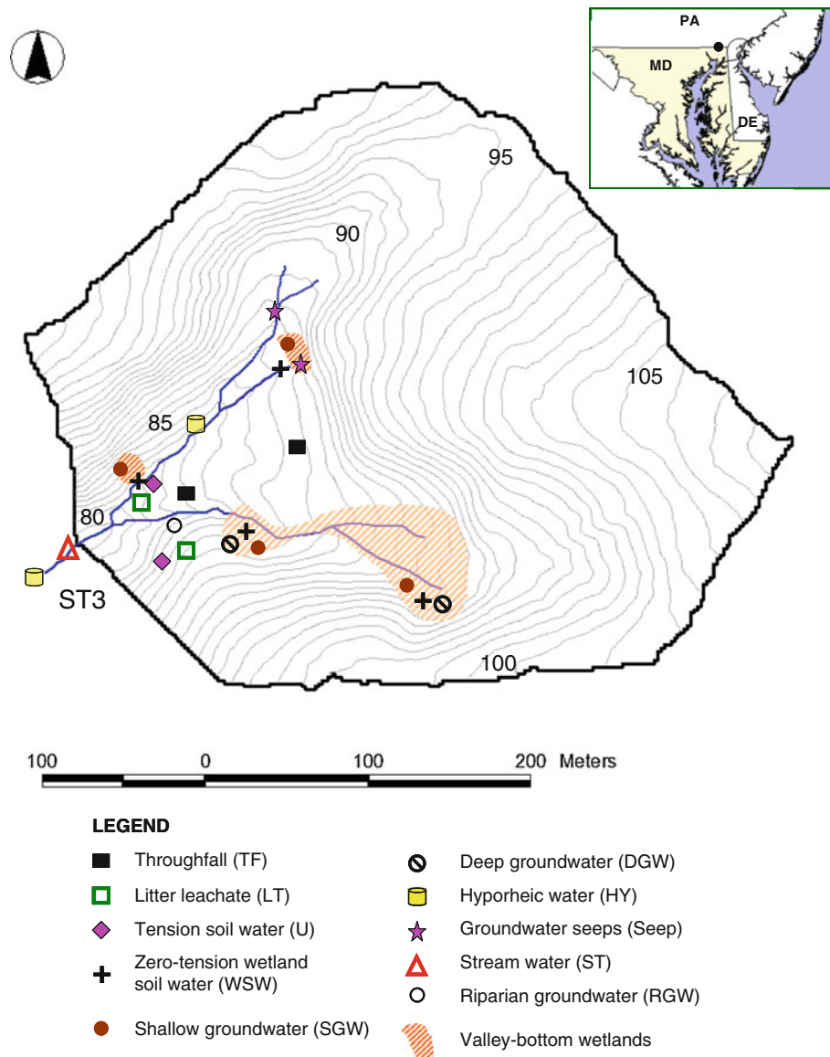
Fig. 1 Location of the study site in the Piedmont region of northeastern Maryland ( inset indicated by filled circle ) and the sampling locations within the 12 ha study watershed
