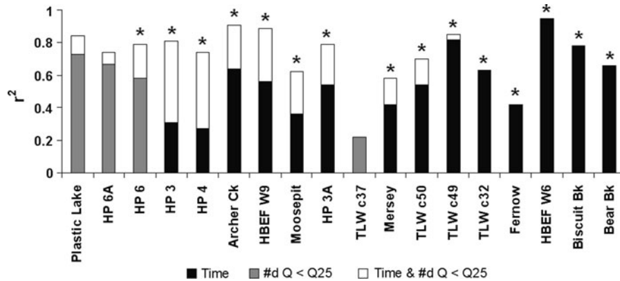
Fig. 5 Comparison of the proportion of variation ( r^2 ) in annual \text{SO}_4^{2-} concentration explained by either time, seasonal dryness (# d Q < Q_{25} ), or time and seasonal dryness in streams from highest (left of x -axis) to lowest (right of x -axis) \text{SO}_4^{2-} response score (* indicates streams where there was a significant temporal
