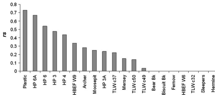
Fig. 4 Comparison of \text{SO}_4^{2-} response scores for 20 catchments in southeastern Canada and the northeastern USA
