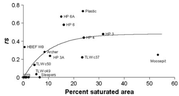
Fig. 8 The relationship between percent saturated area and \text{SO}_4^{2-} response score. Shaded area r_s of 0 and percent saturated area of 0 (TLW c32 and HBEF W6), 0.65 (Bear Brook), 0.87 (Fernow), 1.28 (Biscuit Brook) and 2.15 (Hermine). Note: no % saturated area calculated for Mersey watershed due to corrupted DEM
