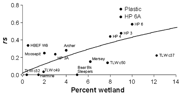
Fig. 7 The relationship between percent wetland coverage and \text{SO}_4^{2-} response score. Open circle symbol represents values ( r_s = 0 and wetlands = 0) for the Biscuit Brook, Fernow and HBEF W6 catchments
