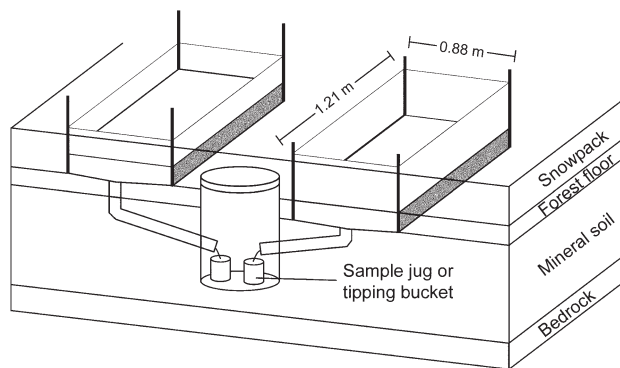
Fig. 1. Schematic diagram of snowmelt and forest floor lysimeters.
