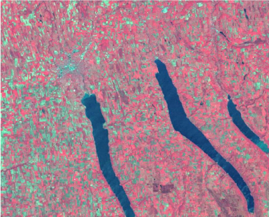
Landsat 1, Path 17, Row 30, Band 7, 5, 4
