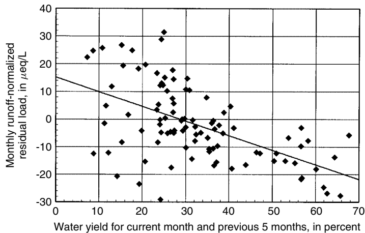
Figure 8. Water yield for period of previous 5 months and current month versus runoff-normalized \Phi_\epsilon for alkalinity. Linear trend-line has R^2 of 0.31
