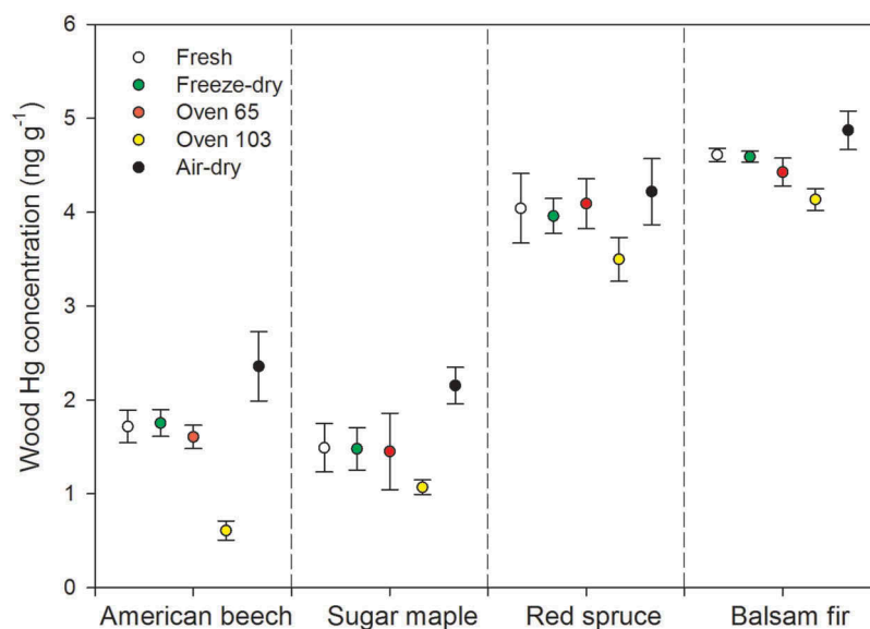
Figure 1. Corrected Hg concentrations measured in samples from four trees of different species prepared by five different methods. Oven-drying at 103°C results in Hg loss, while air-drying results in Hg gain.
