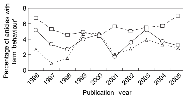
Figure 2. The percentage of articles published in three primary conservation journals that used the term 'behaviour' in their titles or abstracts from 1996 to 2005. B : Conservation Biology, · : Biological Conservation 6 : Ecological Applications
