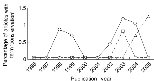
Figure 1. The percentage of articles published in three primary behaviour journals that used the term 'conservation' in their titles or abstracts from 1996 to 2005. B : Animal Behaviour, · : Behavioral Ecology and Sociobiology 6 : Behavioral Ecology and Sociobiology
